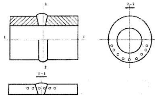
Fig. 8.3.4.6 Examples of hardness test for butt joints in pipe
