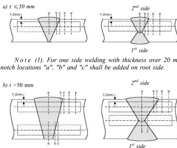
Fig. 6.4.4.3 Location of V-notch for butt weld of high heat input (heat input > 50 \text{ kJ/cm} ):
